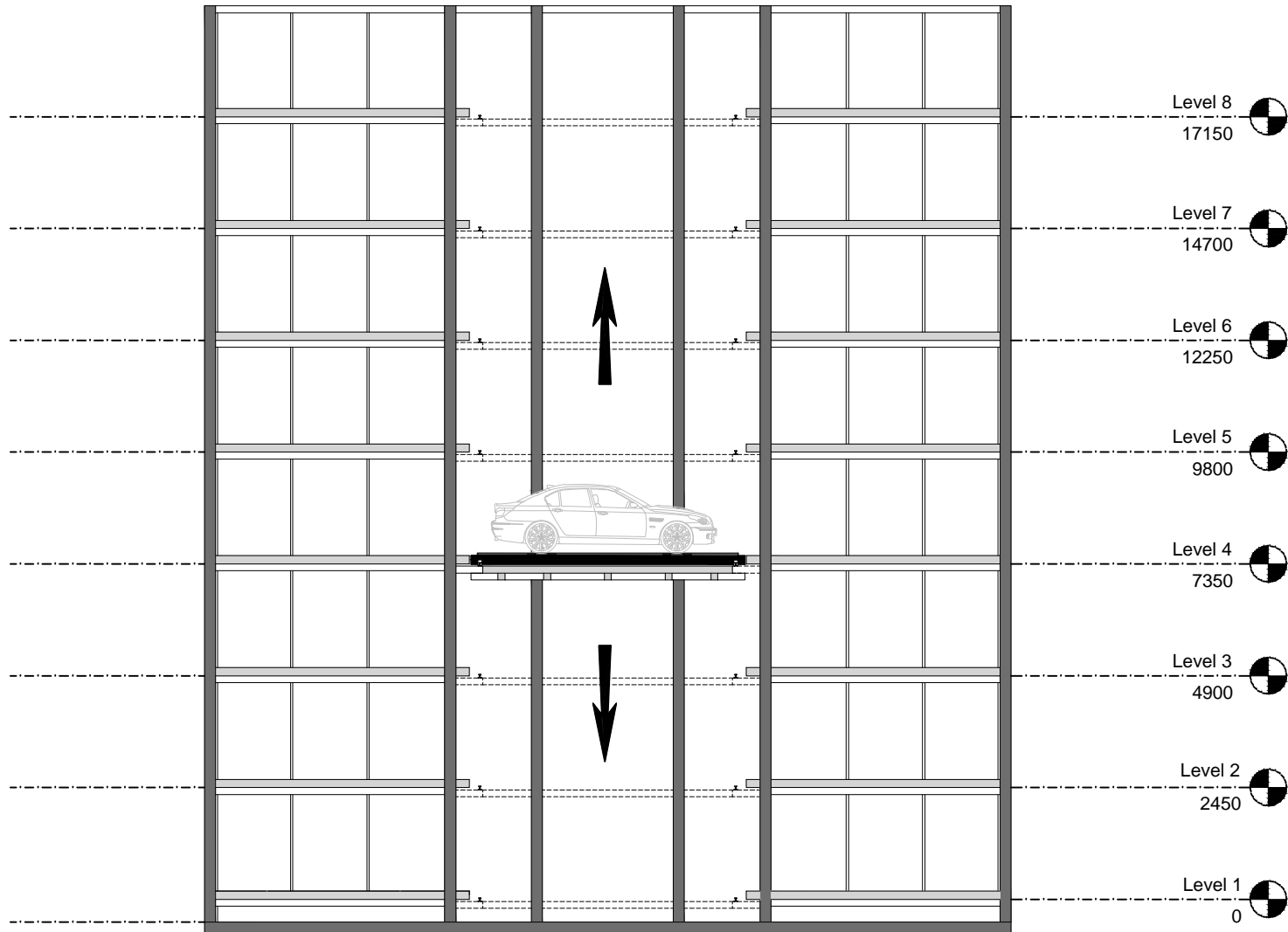
DMT SECTION VIEW
