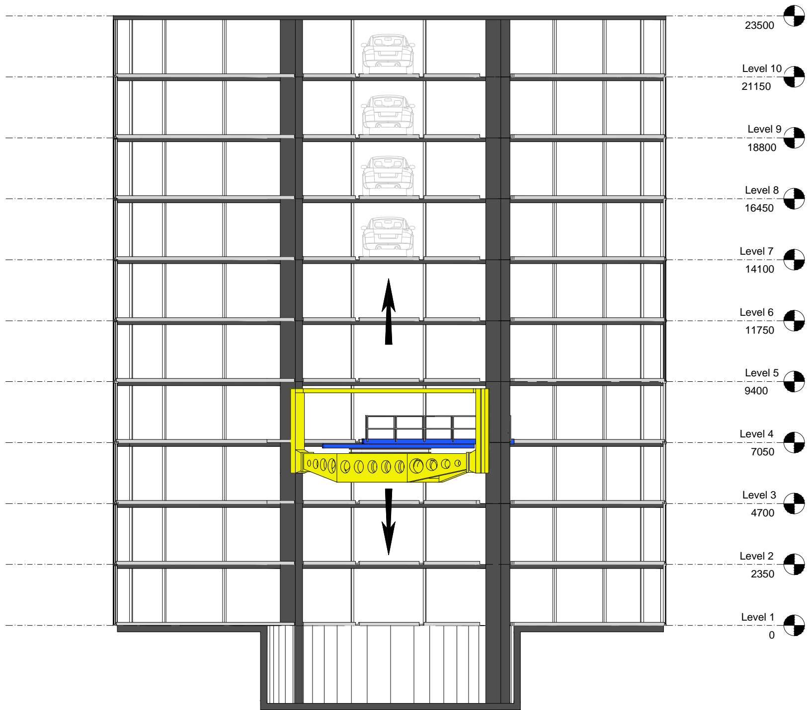
DPT SECTION VIEW
